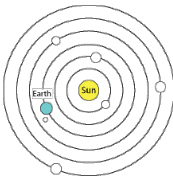
Copernicus’ model 4
