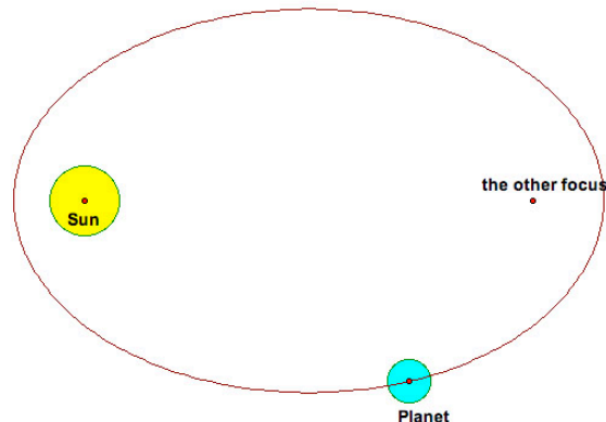
Kepler’s model 5
